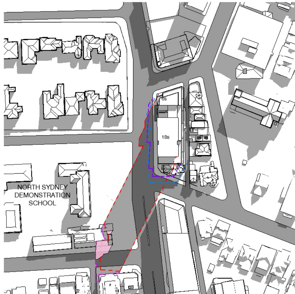
SHADOW DIAGRAM_June21_1100
