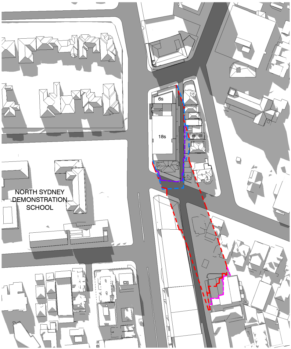
SHADOW DIAGRAM_June21_1400
